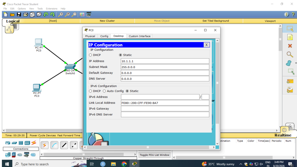
Fig 2: IP configuration of PC0
