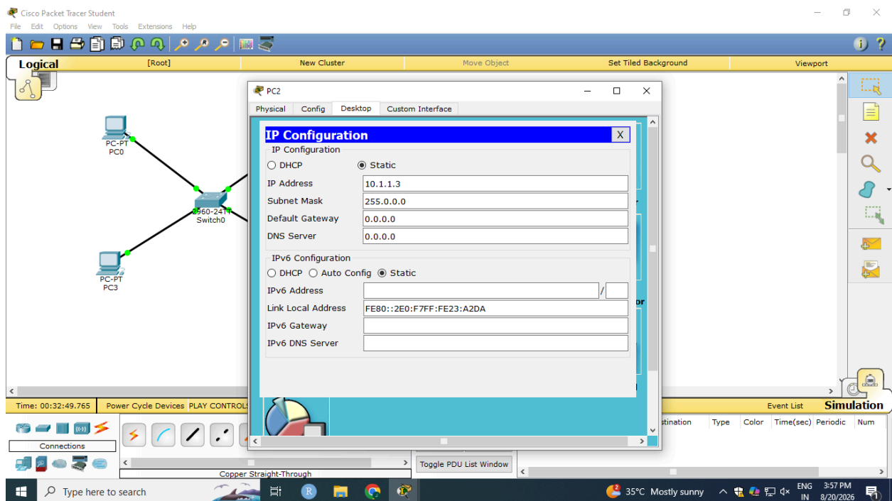
Fig 4: IP configuration of PC2
