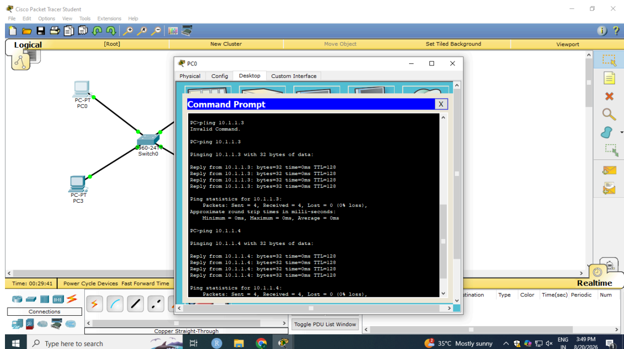
Fig 6: Successful connectivity between PCs in the LAN
